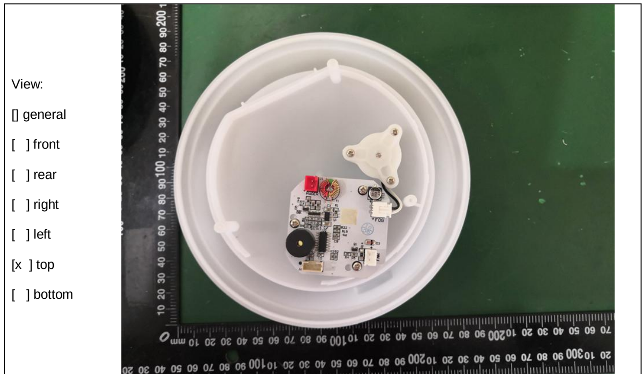
Figure 7. Internal view of unit
