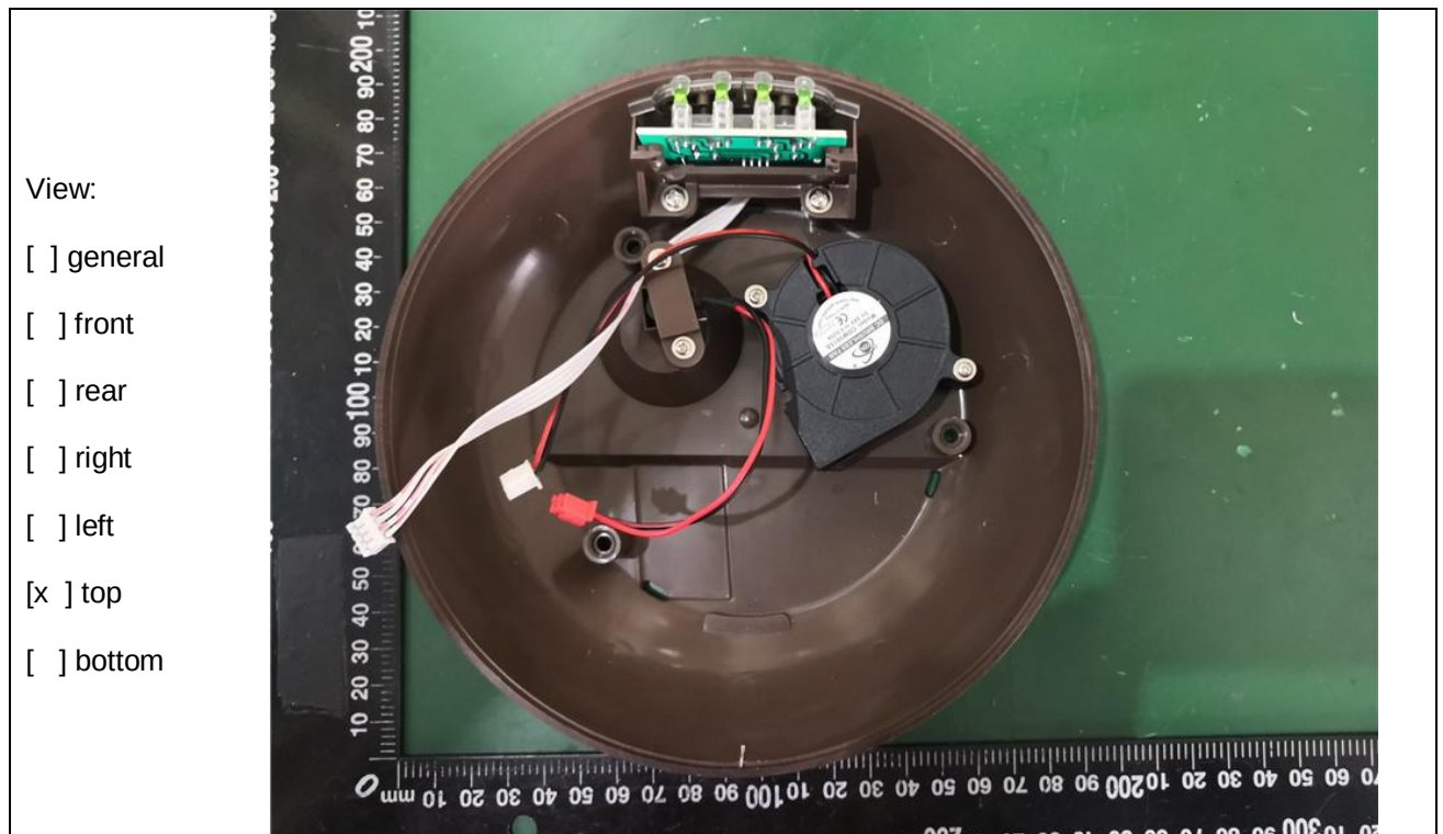
Figure 13. Internal view of unit
