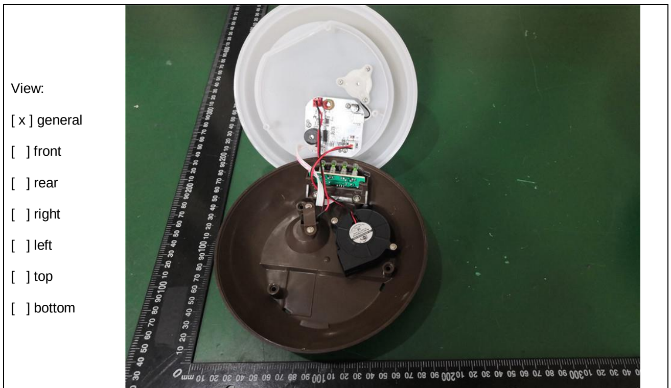
Figure 6. Internal view of unit
