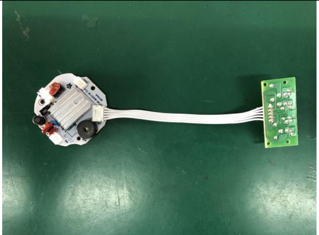
Figure 11. Top view of PCB
