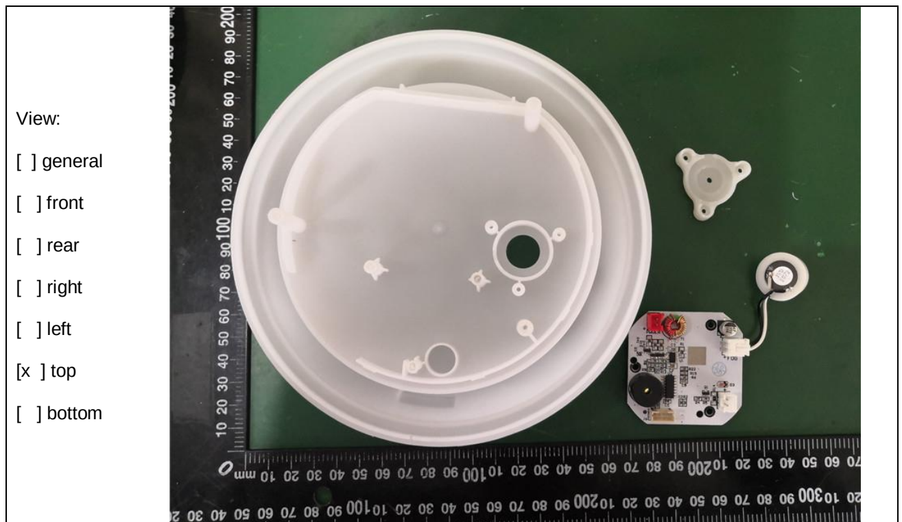
Figure 8. Internal view of unit
